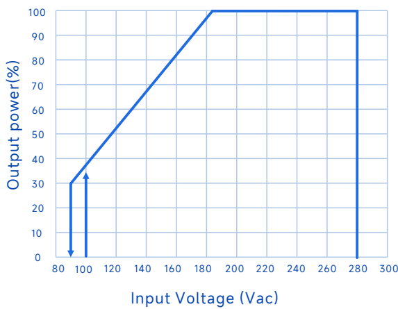
AC Dimming Curve
